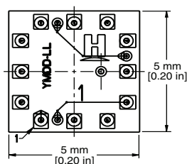
FIGURE 2. PAD FUNCTIONS
